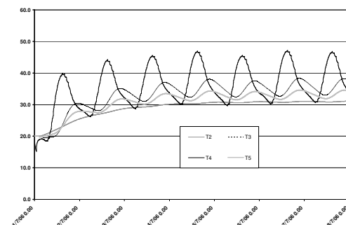
Fig 11. Temperature profile for saturated green-roof, during one week of July.
