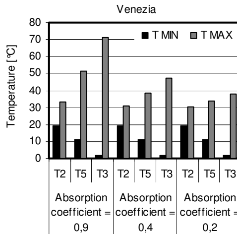
Fig 10. Temperature at 6,8 cm (T2), at 3,8 cm and at 0,8 cm under the external roof surface, for different absorption coefficient.
